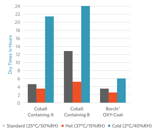
Through Dry Time Comparison of SB Wood Stain
