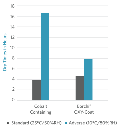
Through Dry Time of SB Pigmented Direct to Metal Applications
